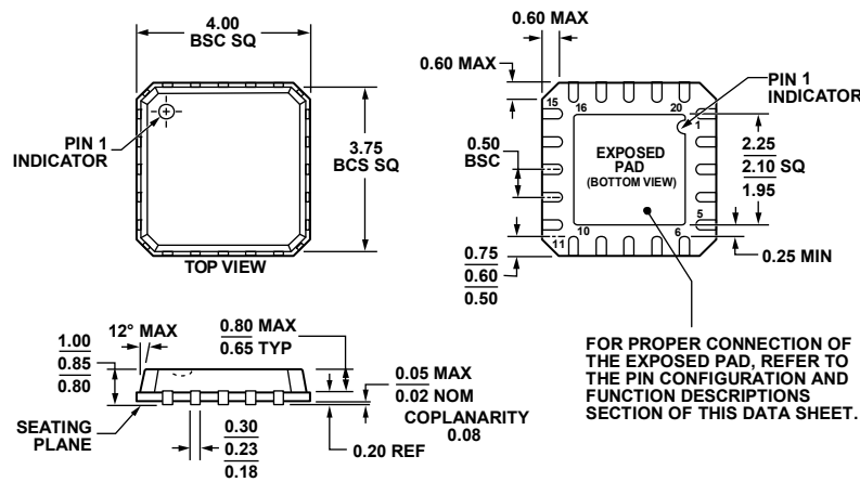
Figure 26. 20-Lead Lead Frame Chip Scale Package [LFCSP_VQ]
