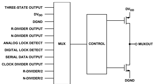
Figure 15. MUXOUT Schematic
